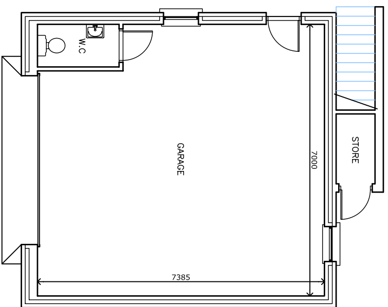
....ground floorplan
