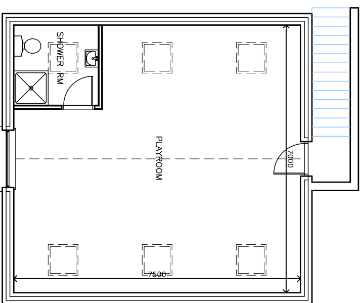
....first floorplan
