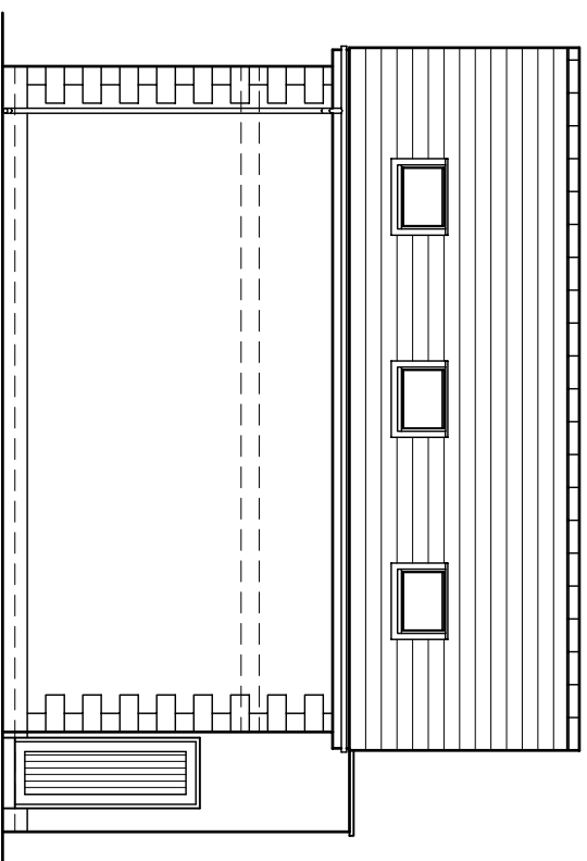
....side elevation
