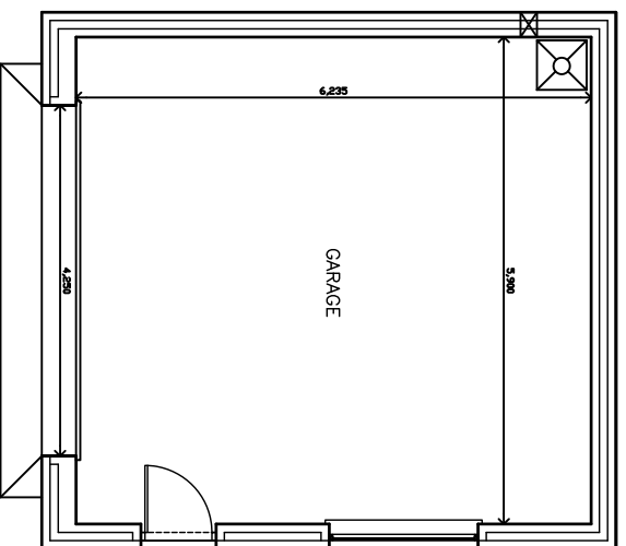
.....floorplan
