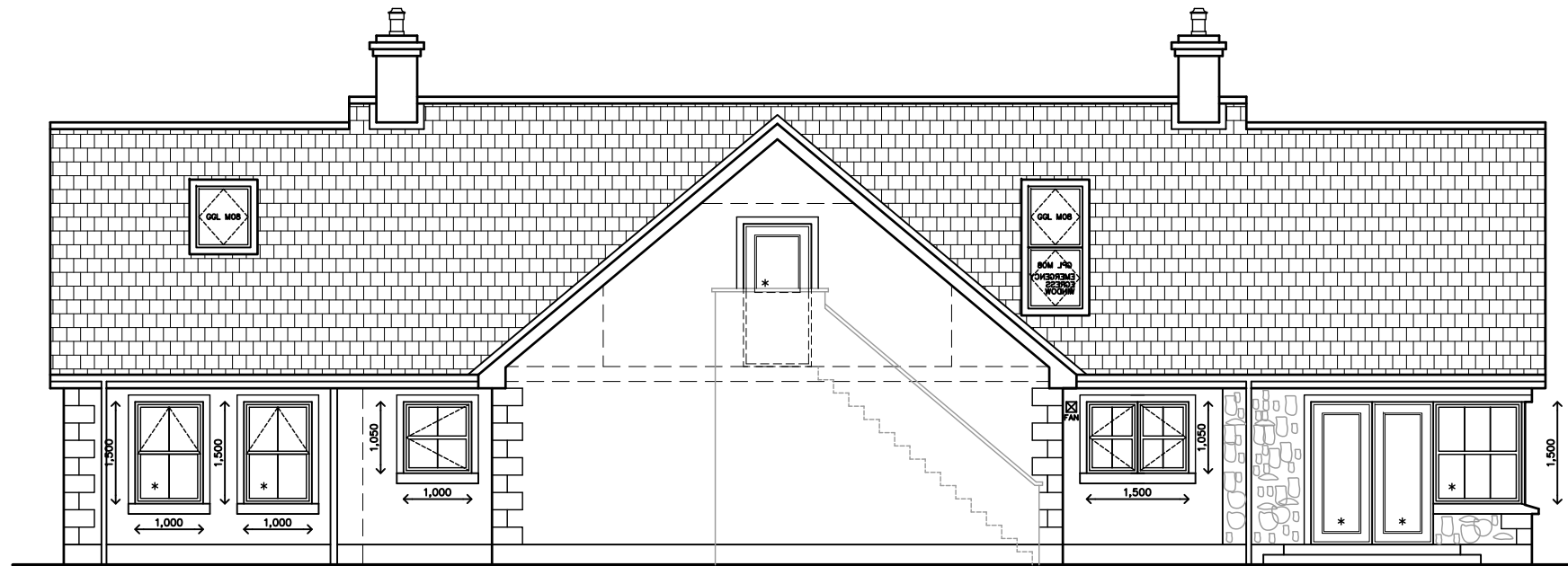
....rear elevation
